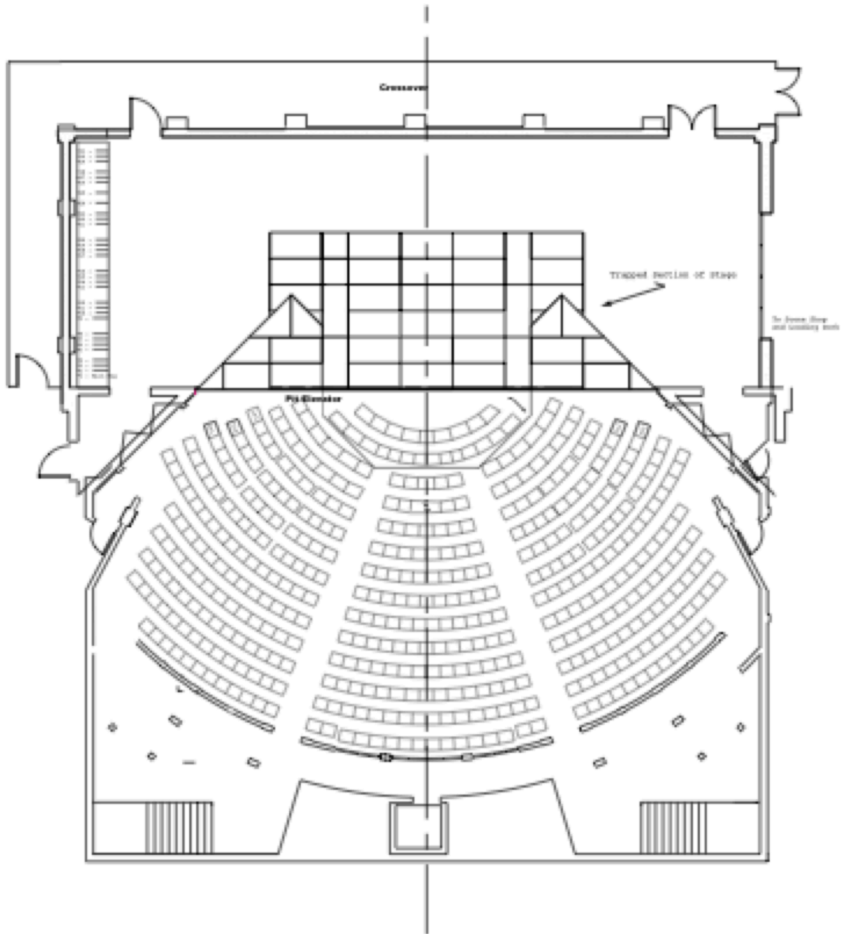
FIGURE 4.3-1 – Alice Jepson Theatre Ground Plan
