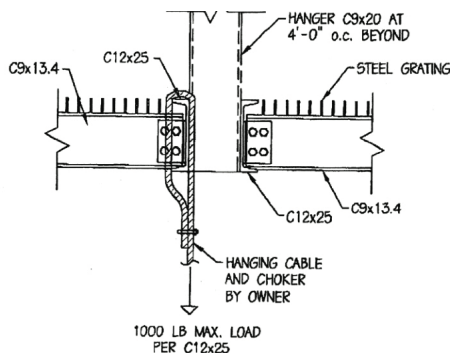
SECTION 1 3/4" = 1'-0"
