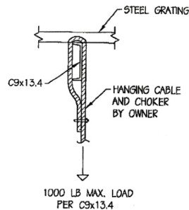
SECTION 2 3/4" = 1'-0"
