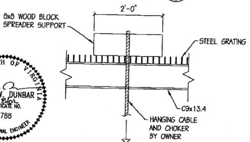
SECTION 1 3/4" = 1'-0"
