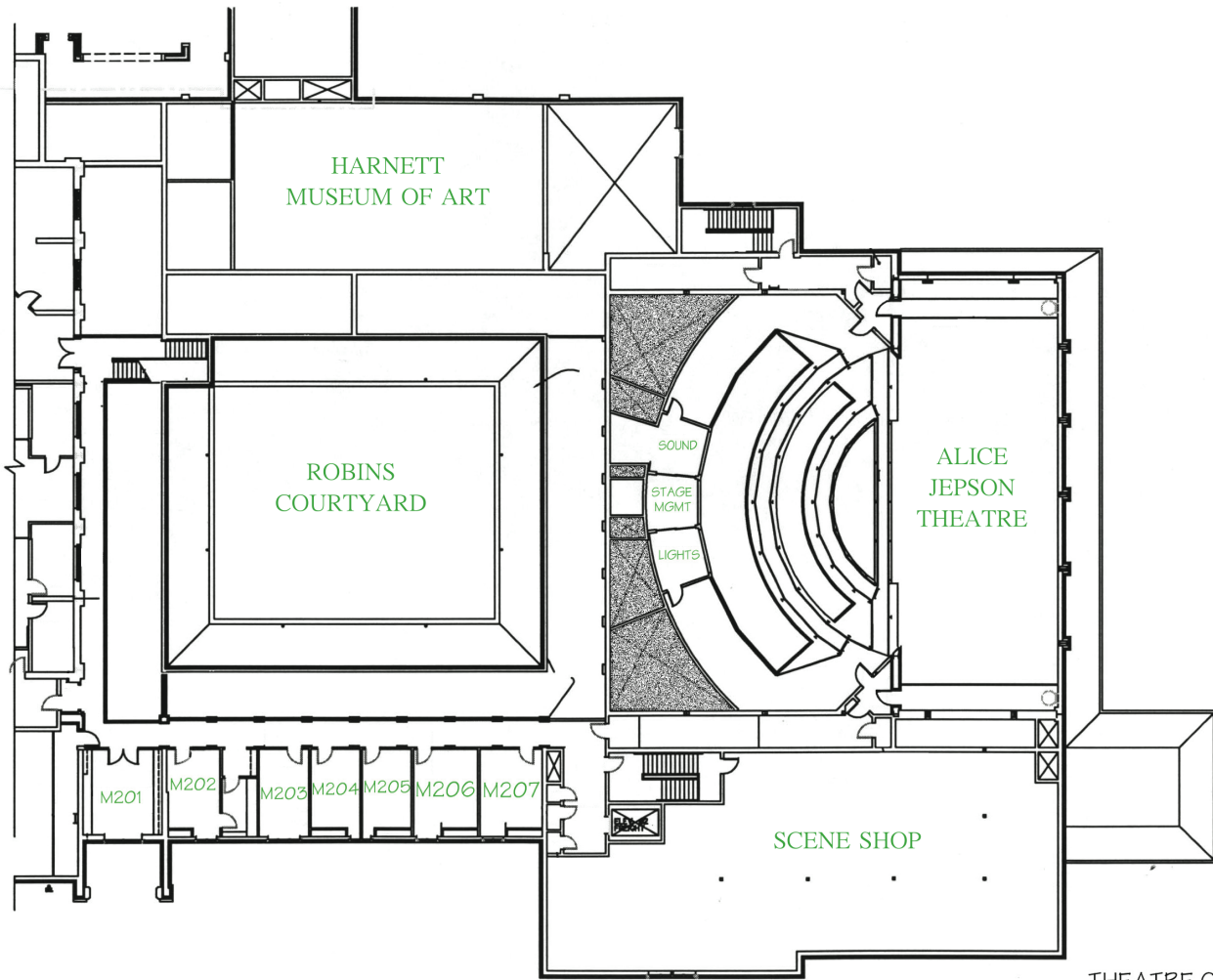
THEATRE COMPLEX SECOND LEVEL PLAN ELEV. @ 214.72' (EXCEPT WHERE NOTED OTHERWISE) SCALE: 1/8" = 1'-0"
