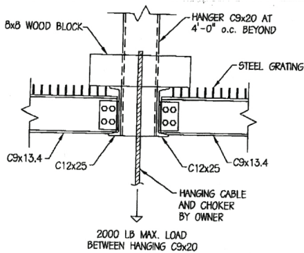
SECTION 1 3/4" = 1'-0"
